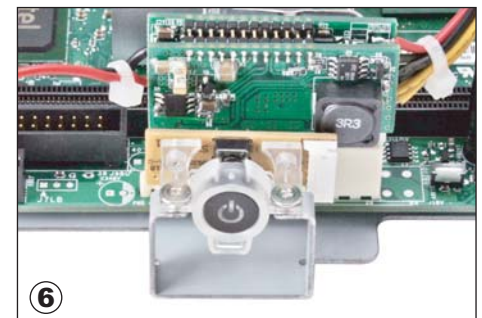
For HDD cage need to fix 2 screws on chassis.
