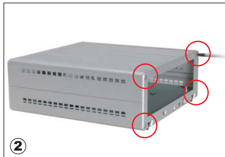
Unscrew 4 screws on the back of chassis.
